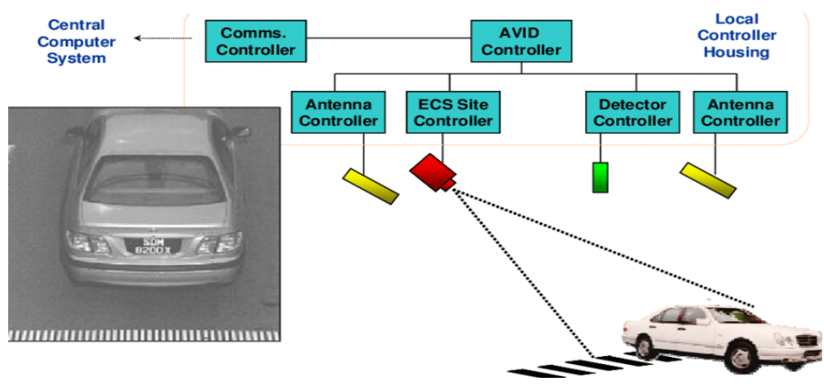
Fig. 2: Installed Gantries which Record Car Movement in ERP
